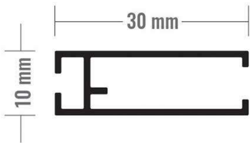
A PROFILE
