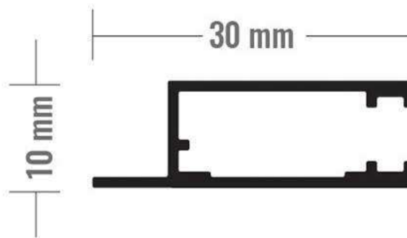
H PROFILE
