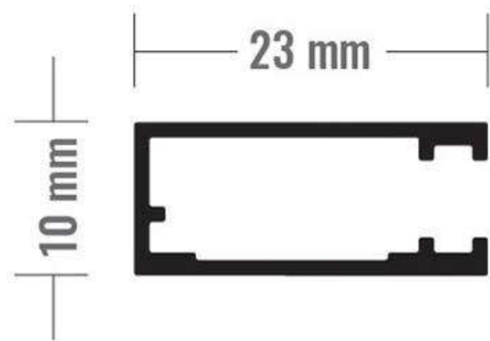
C PROFILE
